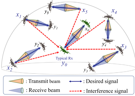
Fig. 1. Directional UAV networks.
